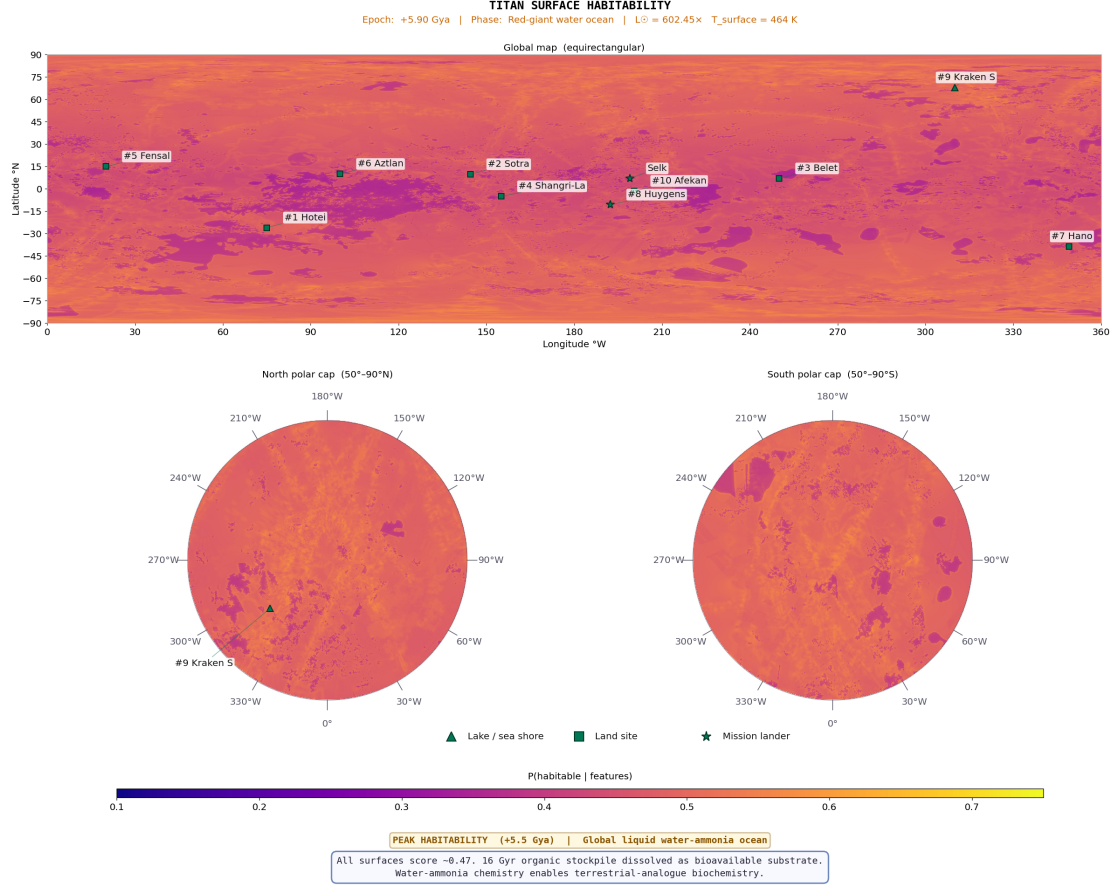
Figure 3.8: Future epoch (+5.9 Gya; red-giant ocean) posterior mean habitability. f_1 and f_8 overridden to 1.0 globally. Spatial variation reflects f_2, f_5, f_6 differences. Compare with Figure 3.4.
